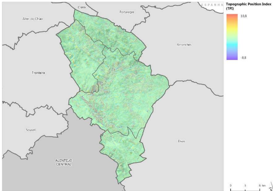
Figura 40. Topographic Position Index (TPI) 48
